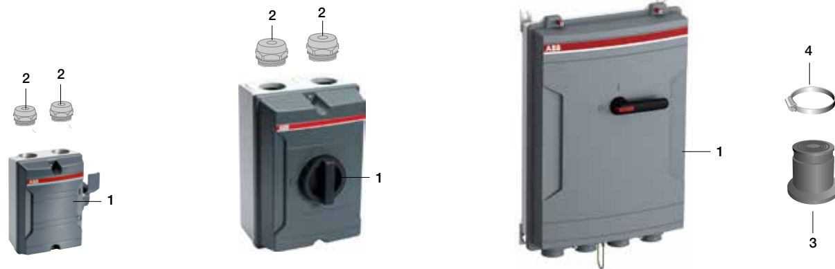
1 Enclosure | 2 Membrane gland/sealing plug (included) | 3 Cable tightening / gland (included) | 4 Hose clamp (included)
