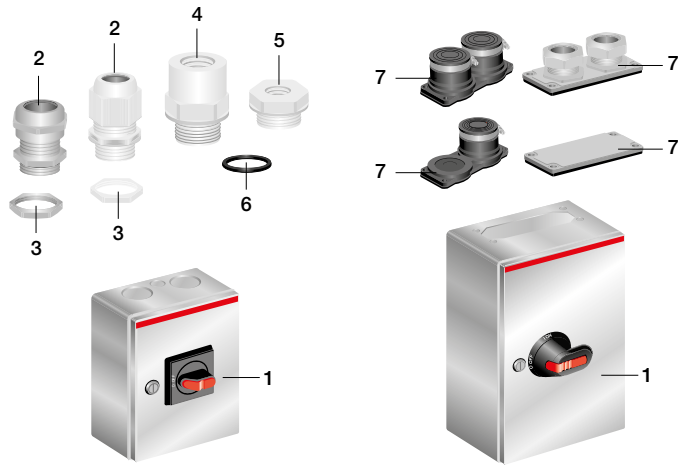
1 Enclosure | 2 Compression gland | 3 Locking nut | 4 Adapter (expander) | 5 Adapter (reducer) | 6 Gasket | 7 B-flange
